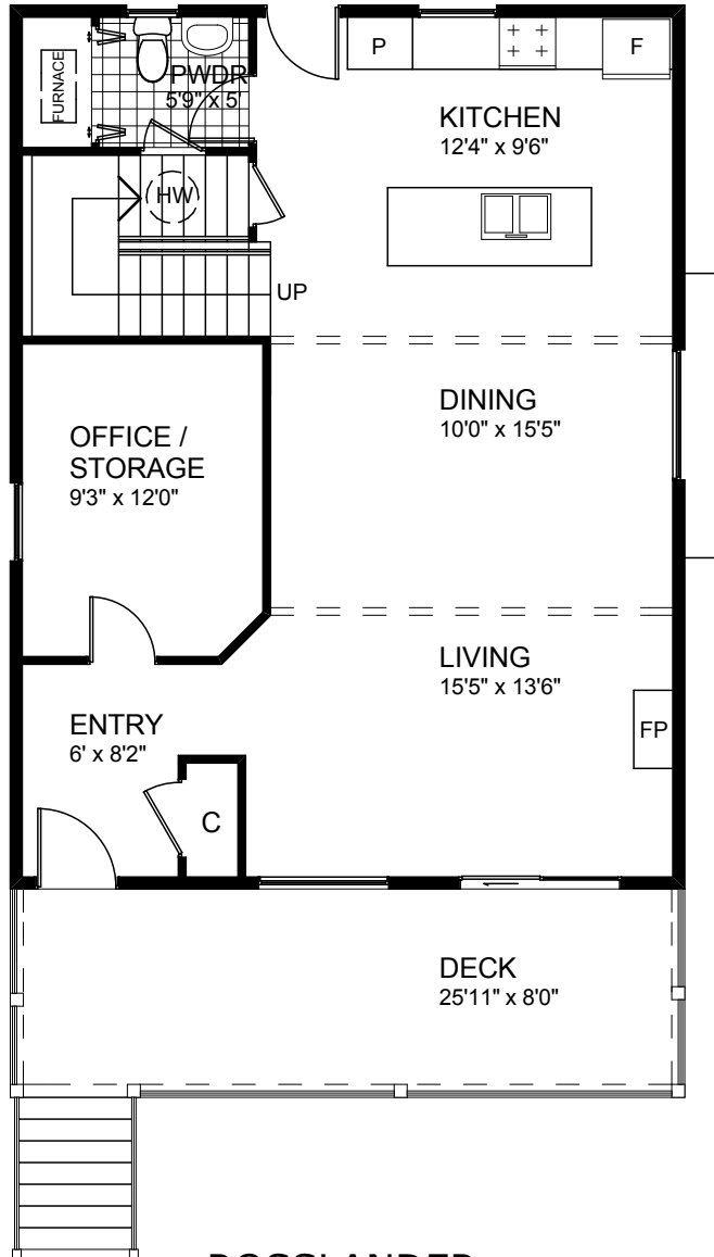
ROSSLANDER MAIN FLOOR 880 SF DECK 207 SF
